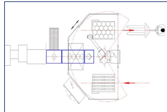
Palletizing for various products Primary and secondary packaging
