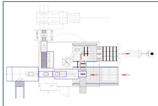
Case packing and palettizing Web press deliveries, finishing, packaging
