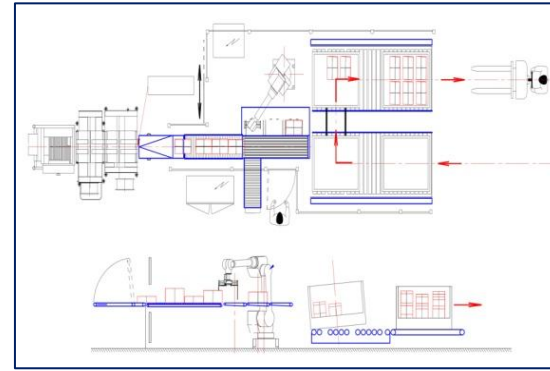
Palletizing in case or on pallet Finishing, addressing
